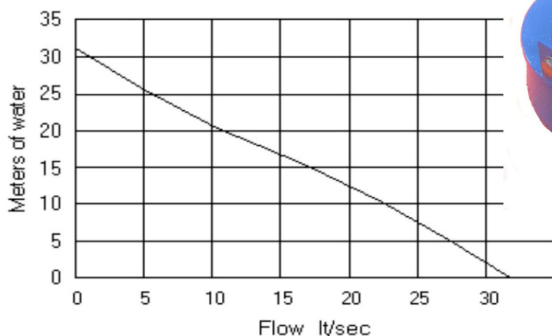
3 INCH SUBMERSIBLE
